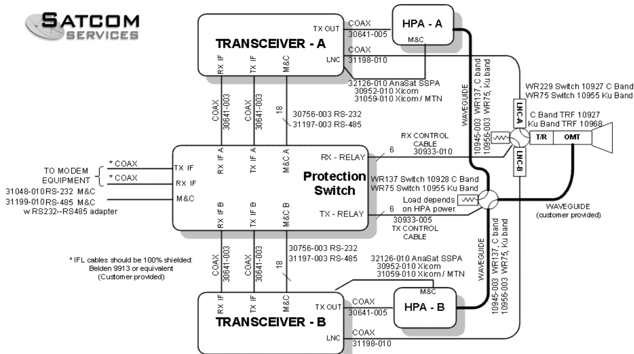
ANACOM 1 + 1 Redundancy Protection Switch Cabling Diagram (External HPA)
